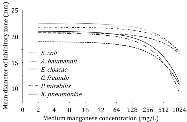
FIG 2 Effect of increasing medium manganese concentrations on average zone diameters, measured by disk diffusion.
