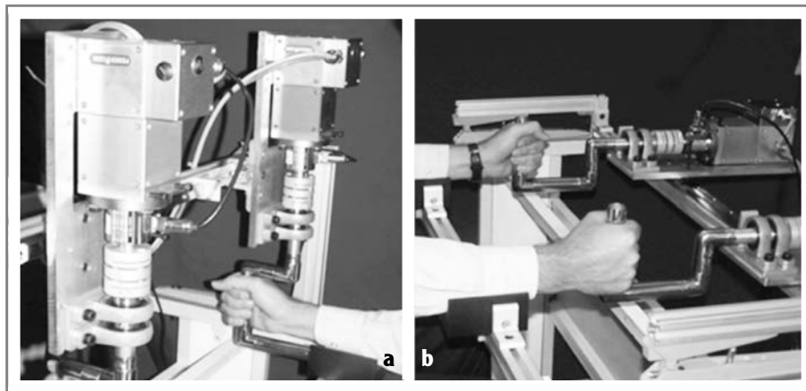
Figure 2.14 Hand robotic rehabilitation device. (a) Wrist flexion and extension. (b) Forearm pro-and supination. Reprinted with permission.
