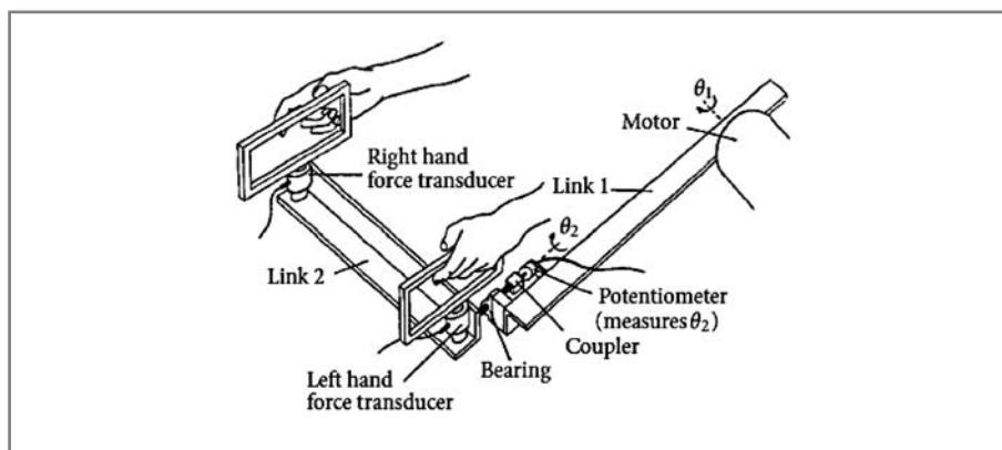
Figure 2.8 The Bimanual Lifting Rehabilitator. Reprinted with permission.
