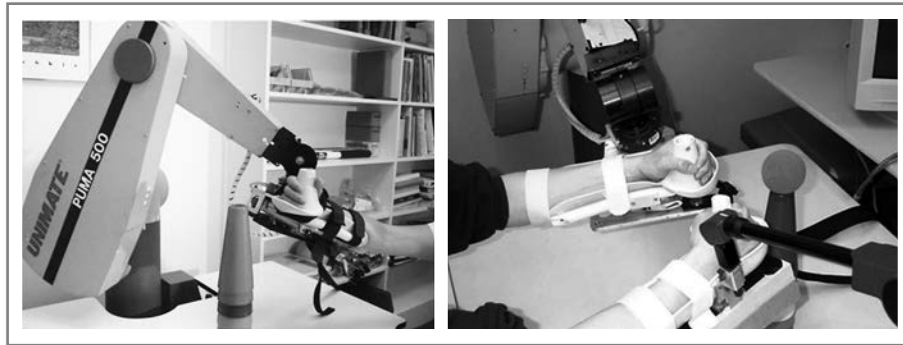
Figure 2.9 MIME. (a) Unilateral mode. (b) Bilateral mode. Reprinted with permission (funding: US Department of Veterans Affairs Rehabilitation Research and Development Program).
