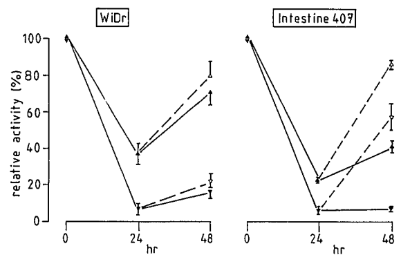
Fig. 7. Recovery of thymidylate synthase in Intestine 407 and WiDr cells. Solid lines (connecting closed symbols) represent the activity in the continuous presence of 5-FU and deoxyinosine (0.4 mM). 5-FU concentrations were 1 and 0.5 \mu M for Intestine 407 and WiDr, respectively. Broken lines (connecting open symbols) represent culture in drug-free medium, after replenishment at 24 h. Values are means \pm S.E. of three separate experiments. \blacktriangledown , \blacktriangledown ; activity of thymidylate synthase assayed at 1 \mu M dUMP ; \blacktriangle , \blacktriangle ; activity assayed at 10 \mu M dUMP .
