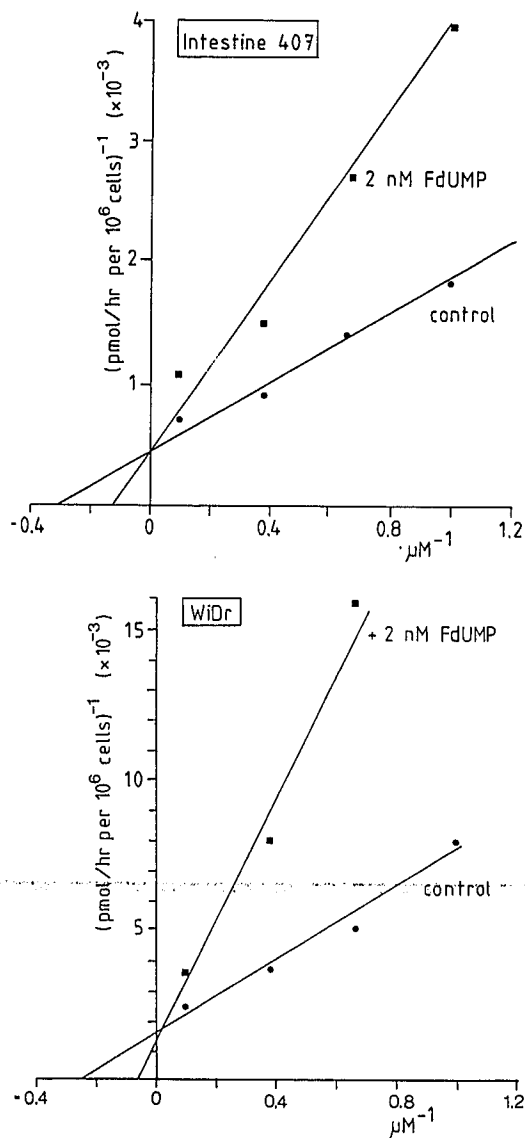
Fig. 6. Lineweaver-Burk plots of thymidylate synthase in Intestine 407 cells and WiDr cells. The K_m values for dUMP were 2.78 \pm 0.34 and 3.72 \pm 0.28 \mu M for Intestine 407 and WiDr cells, respectively, and the K_i values for FdUMP 1.84 \pm 0.35 and 0.50 \pm 0.14 nM respectively. V_{max} values were 1361 \pm 57 and 379 \pm 41 pmol/h per 10^6 cells, respectively. Values are means \pm S.E. of three separate experiments. Enzyme inhibition by FdUMP was competitive in respect to dUMP . The plots are of one representative experiment.
